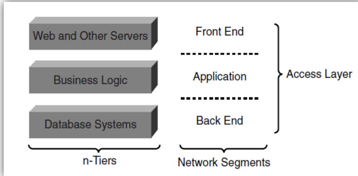
Fig. Multitier Network Segments [4]
