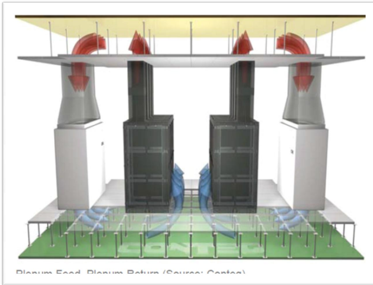
Fig. Closed-Circuit Air Conditioning Operation
