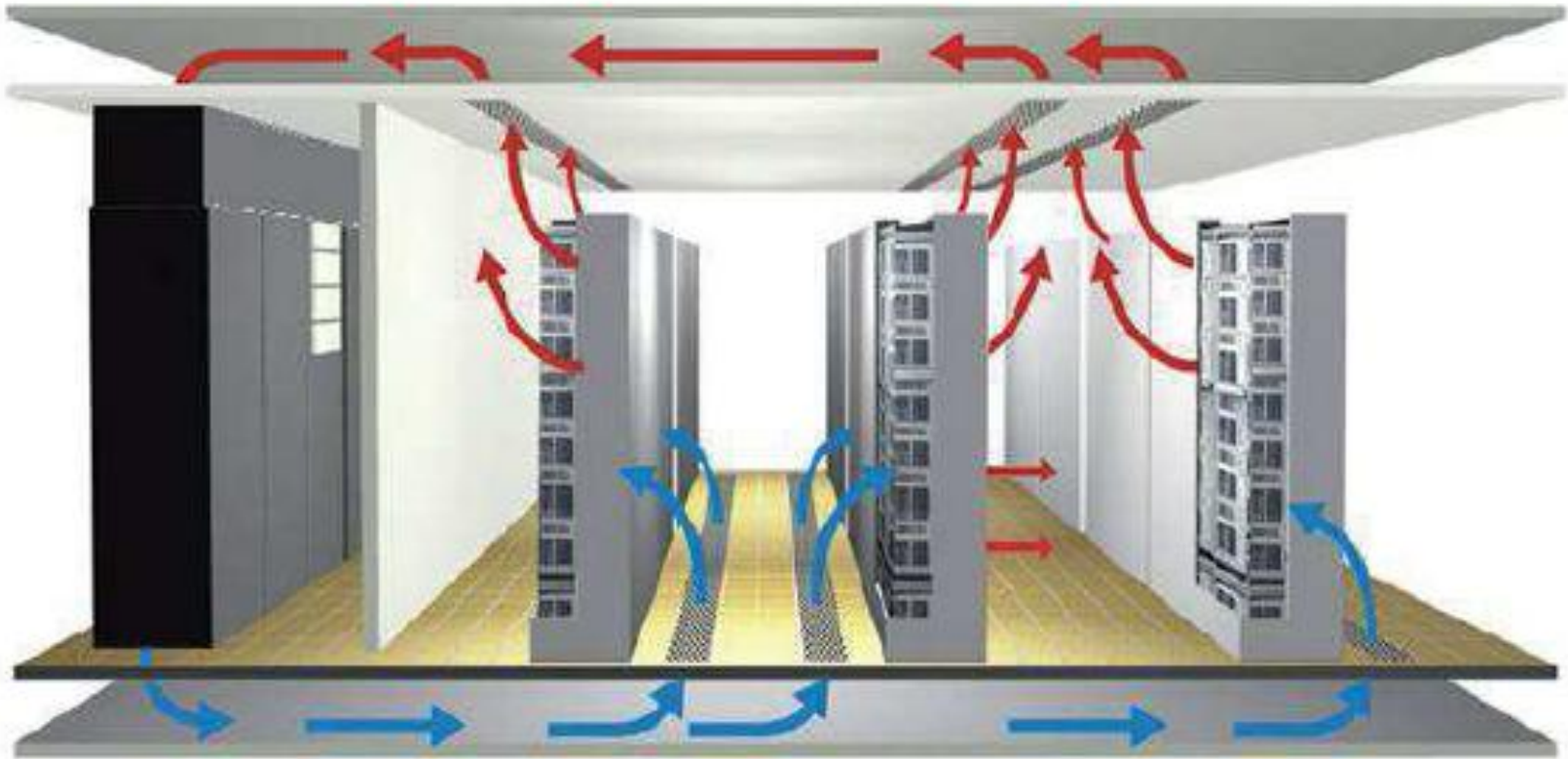
Fig. Solution per the cold aisle/hot aisle principle – closed-circuit air conditioning (Source: BITKOM)
