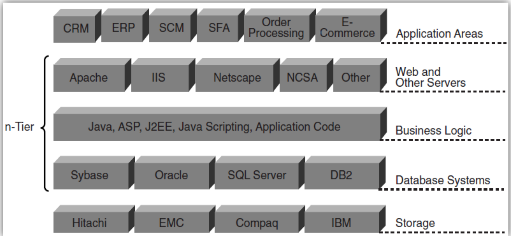
Fig. n- Tier Model [4]
