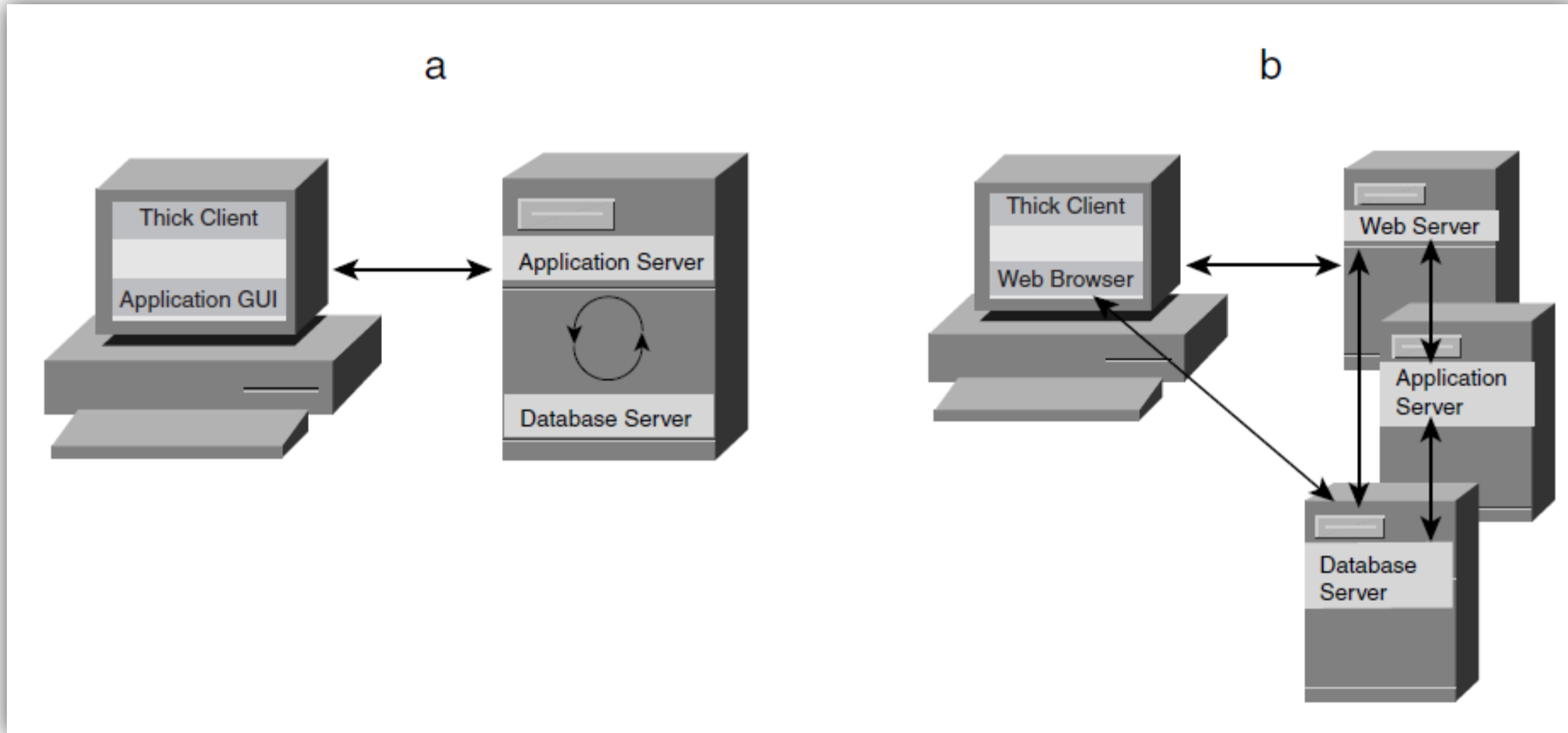
Fig. Client/Server and n-Tier Application Interaction [4]
