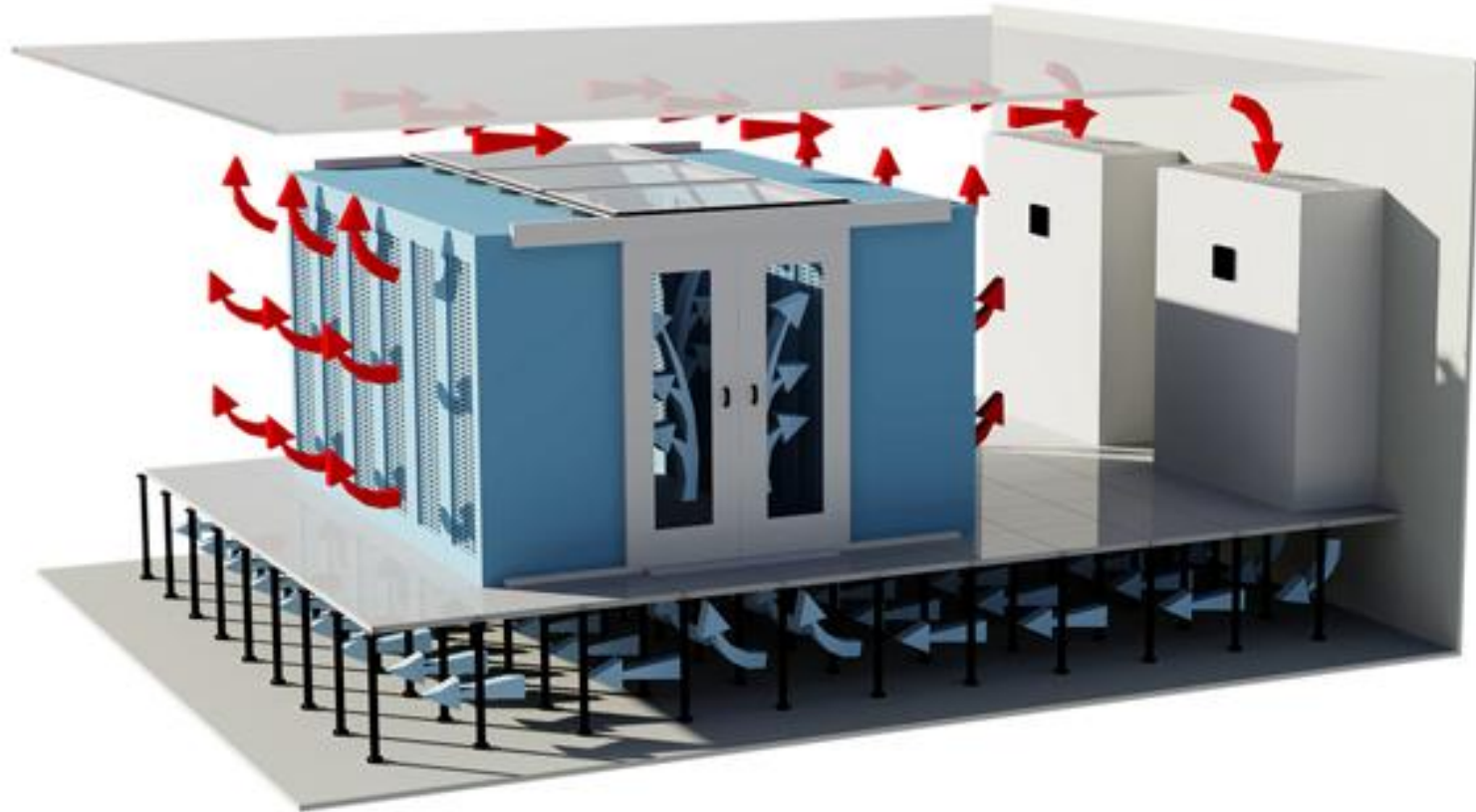
Fig. Cold Aisle Containment
