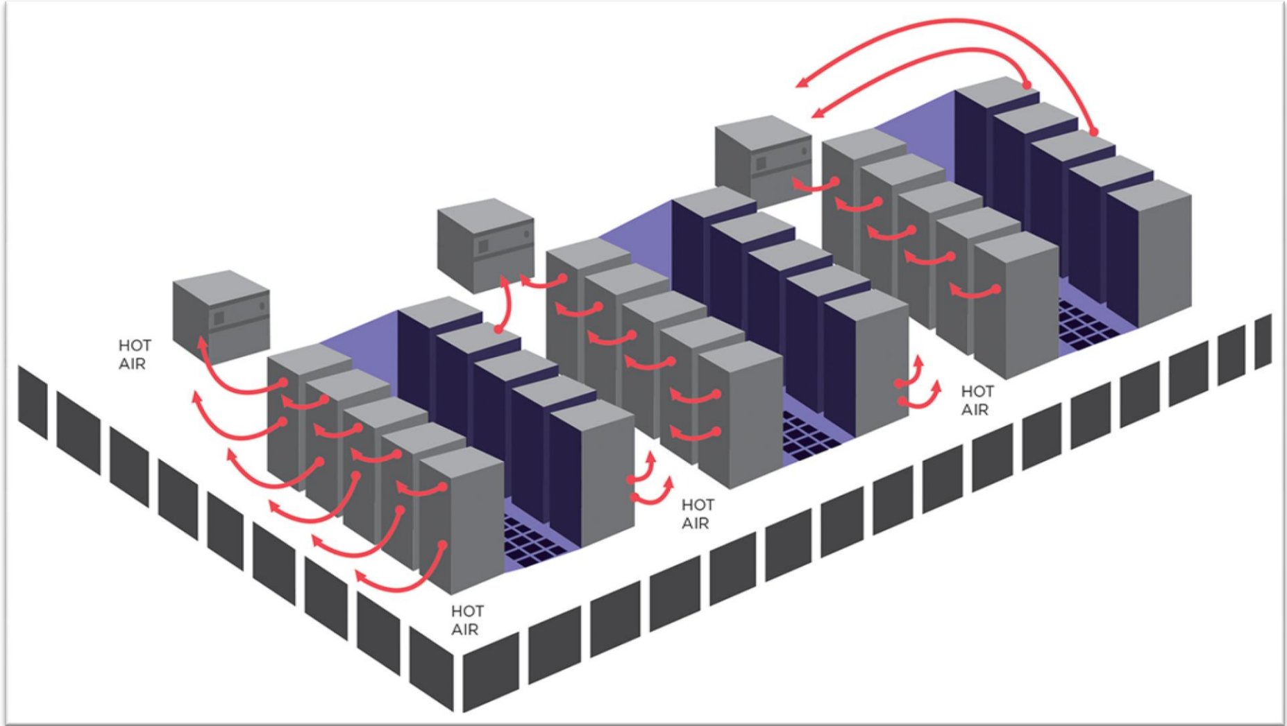
Fig. Cooling, Hot and Cold Aisles
