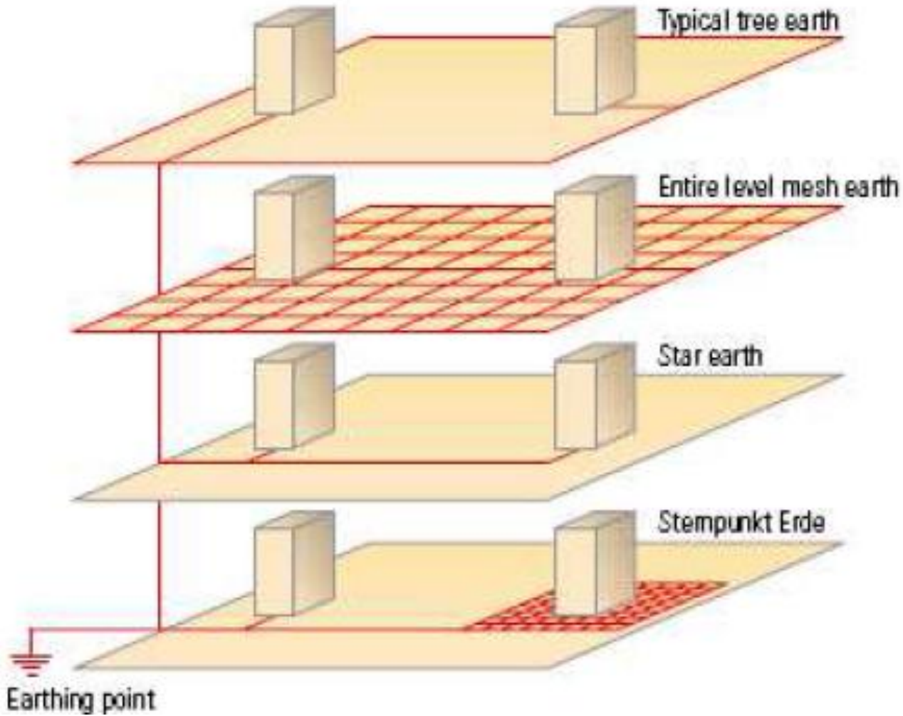
Fig. Grounding System
