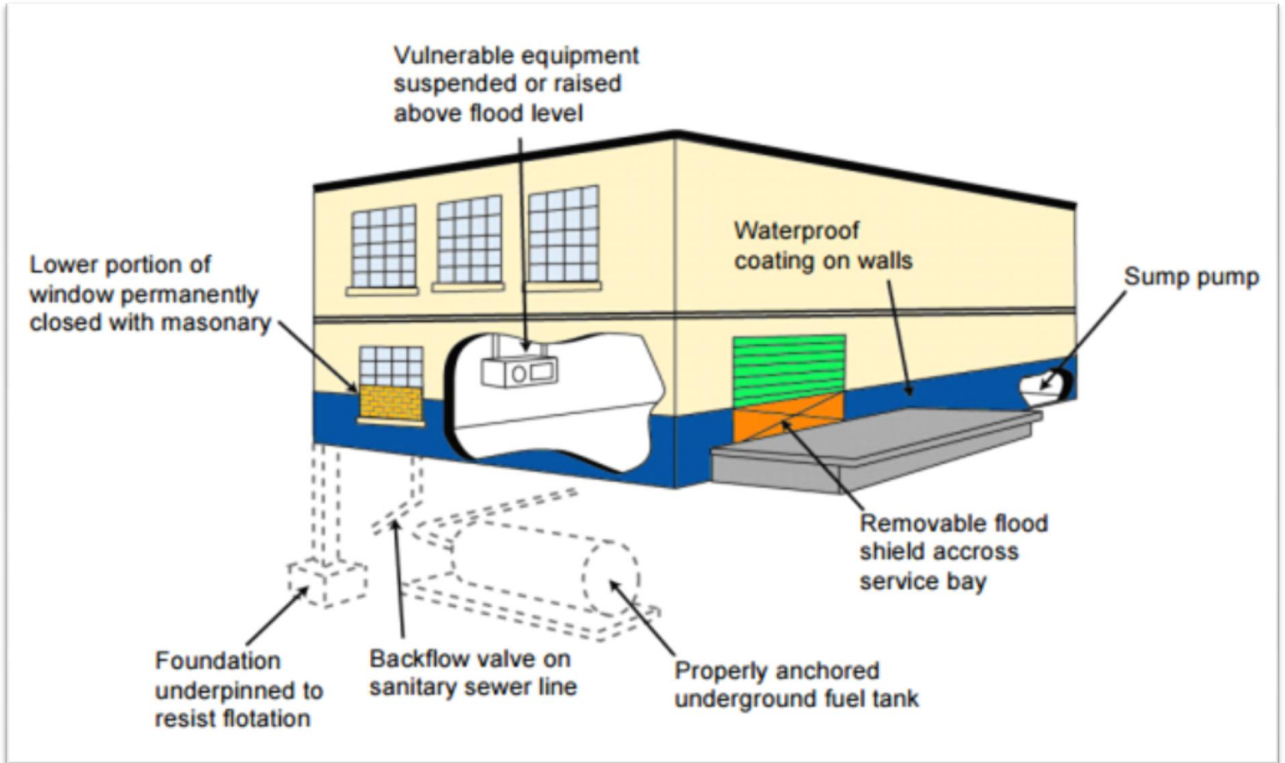
Fig. Dry flood proofing
