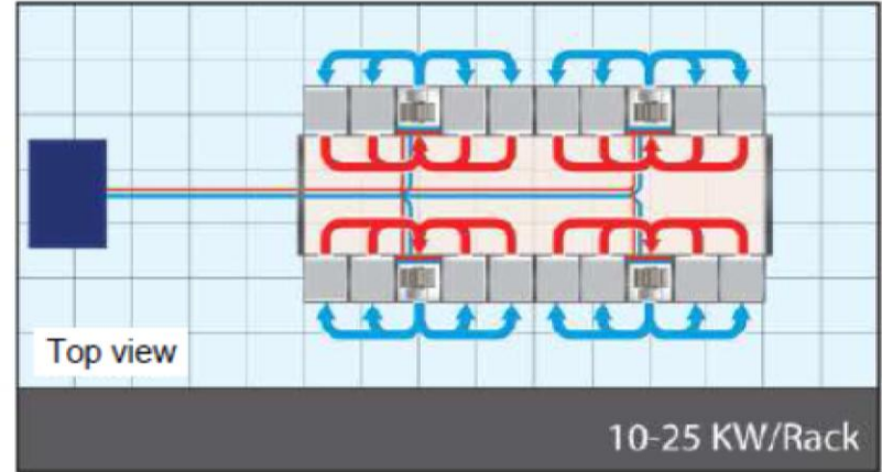
Air conditioning system with water-cooled housing for hot aisles
