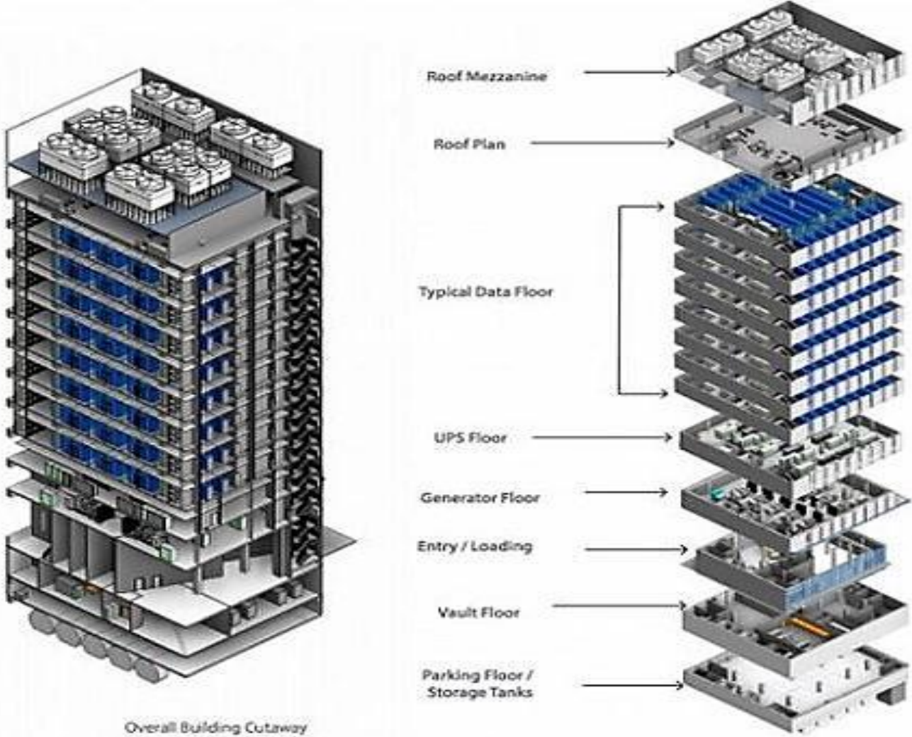
A cutaway of the proposed data center (source: public documents, Seattle.gov)
