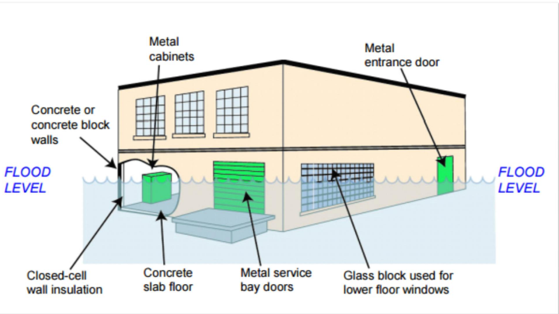
Fig. Flood-resistant materials
